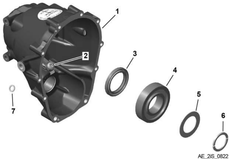
Fig. 1 Gearbox housing with replacement parts (912 i Series)
