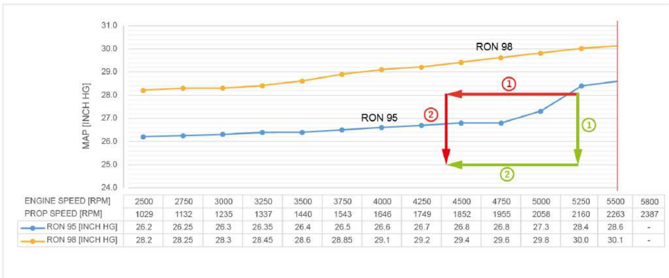
Fig. 3 Power reduction
