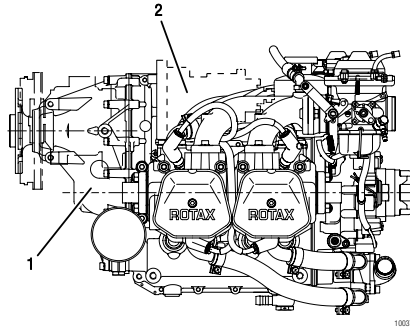
Figure 1: Engine components
