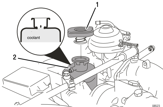
Figure 1: Expansion tank
